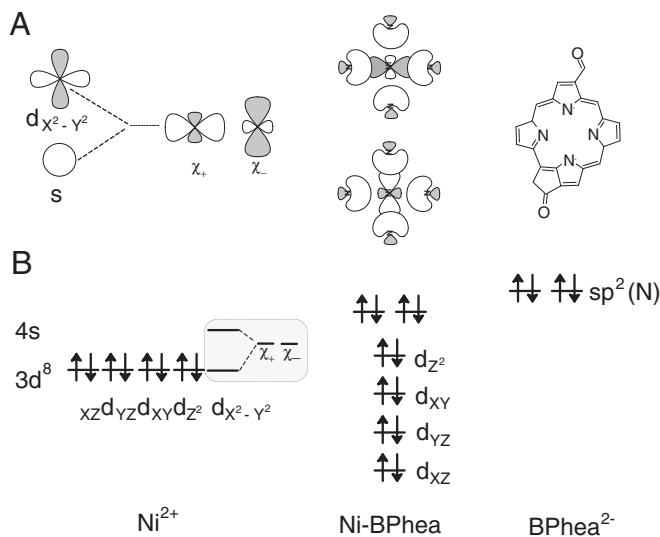
Fig. 6. Schematic presentation of (A) interacting orbitals of Ni^{2+} ion and bacteriopheophytin (BPhe) macrocycle in the complex (no axial ligands present), and (B) the electron occupancy of the orbitals involved, assuming the ligand field of C_{2h}/C_1 symmetry.
